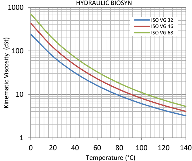
KVT Diagram HYDRAULIC BIOSYN
